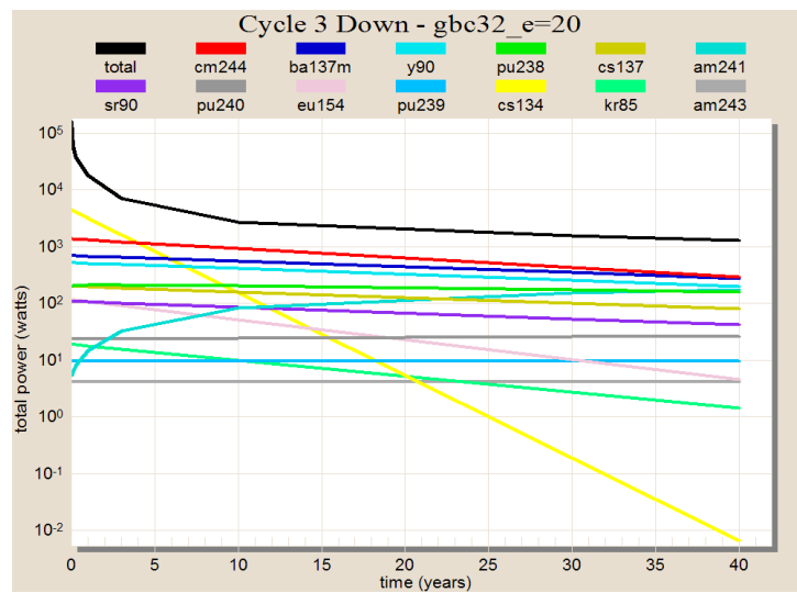
Figure 11: Decay heat primary contributors (e=2.0 w/o)
