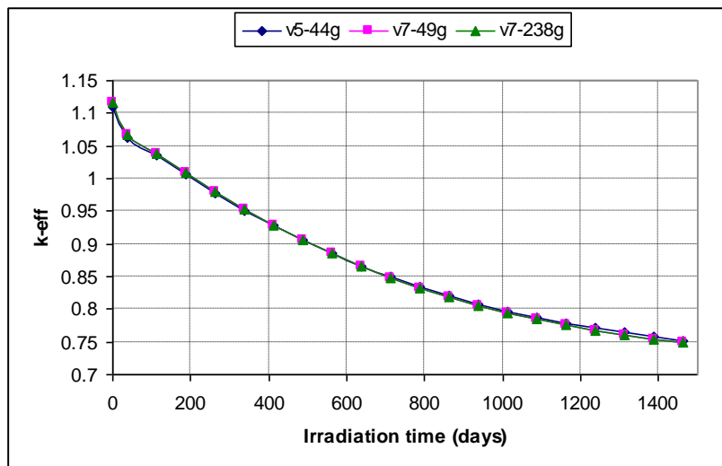
Figure 5: TRITON k-eff depletion results ( e=2.0 w/o)
