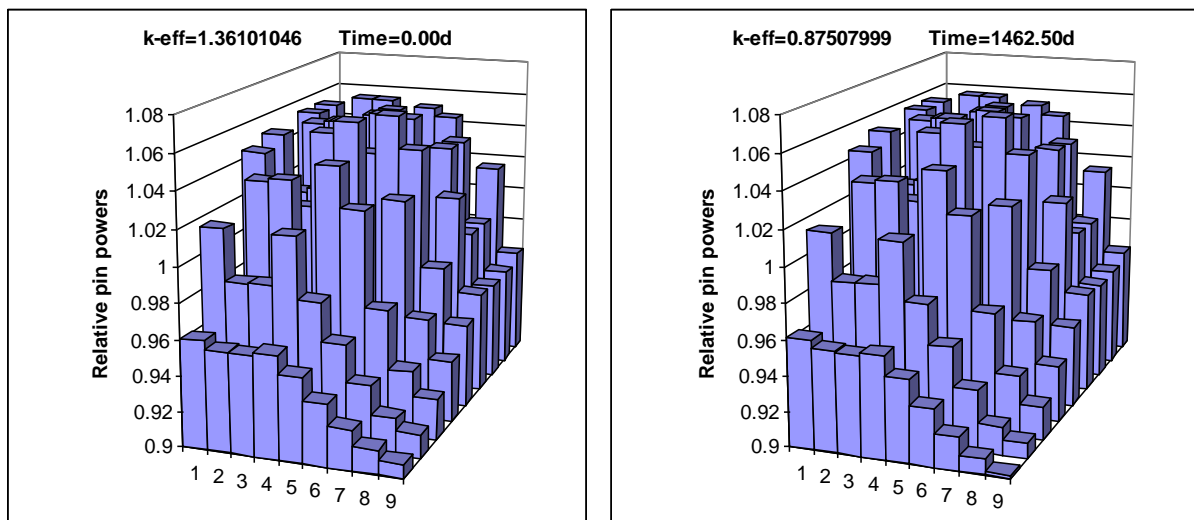
Figure 8: Relative pin power distribution in OFA (e=5.0 w/o)
