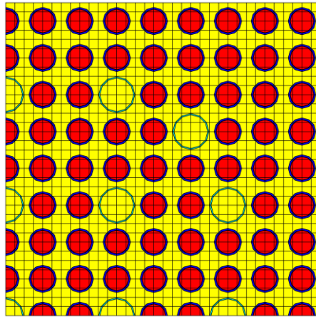
Figure 2: NEWT model of the OFA with SN mesh (1/4 geometry)
