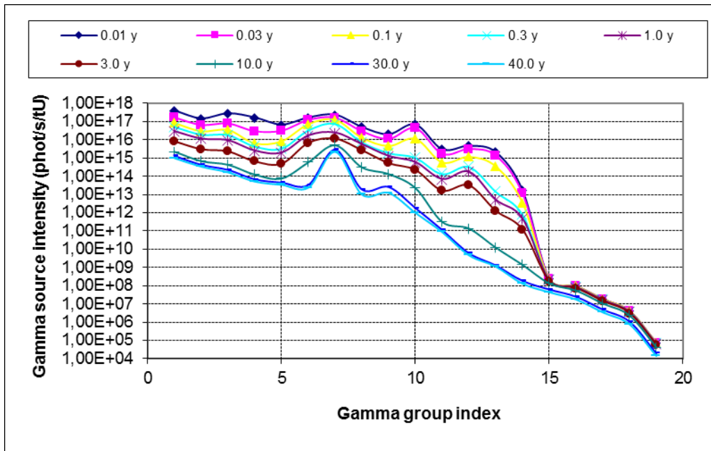
Figure 12: Gamma source intensity (phot/s/tU) for different groups (e=2.0 w/o)
