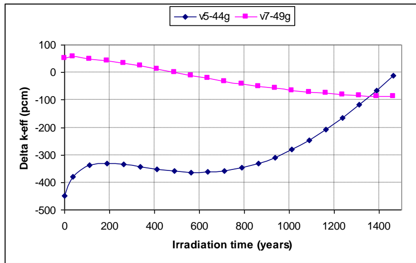
Figure 7: Delta k-eff (pcm) for v5-44g and v7-49g libraries (e=5.0 w/o)
