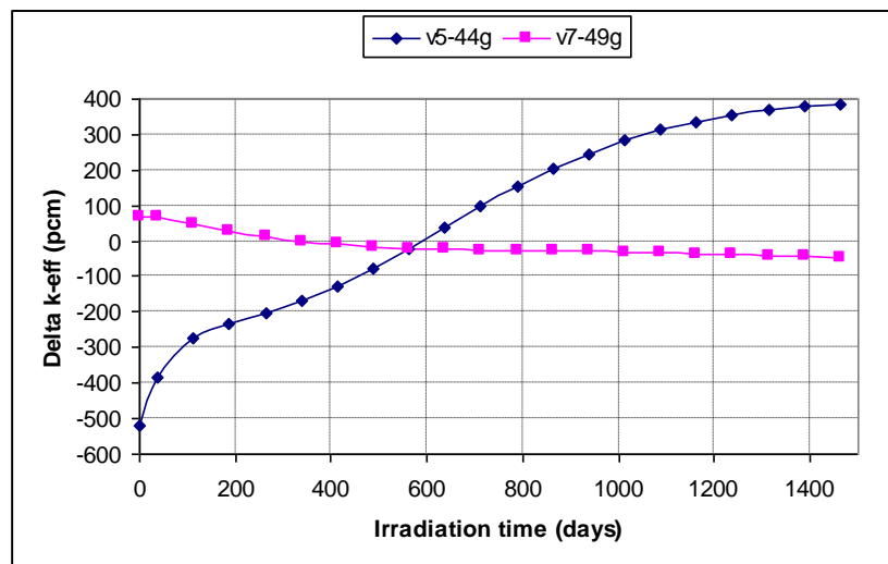
Figure 6: Delta k-eff (pcm) for v5-44g and v7-49g libraries ( e=2.0 w/o)
