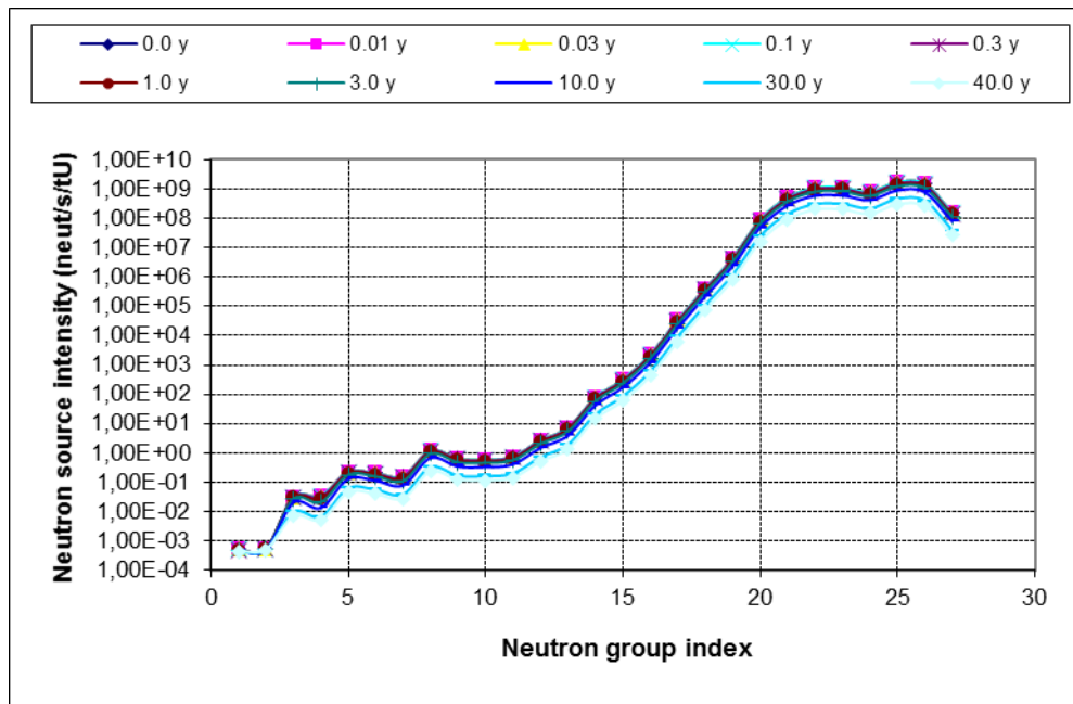
Figure 13: Neutron source intensity (neut/s/tU) for different groups (e=2.0 w/o)
