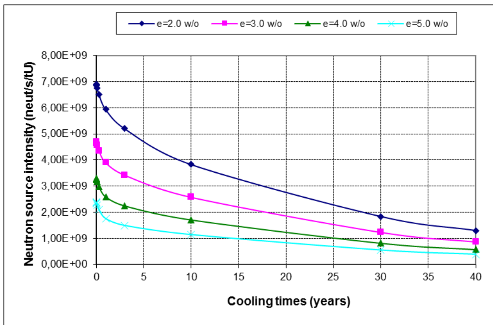
Figure 15: Neutron source intensity (neut/s/tU) as a function of time for different enrichments
