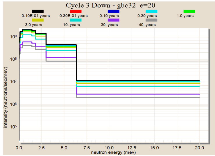
Figure 10: Total neutron spectra in neutrons/s/MeV (e=2.0 w/o)
