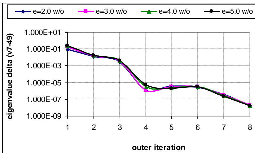
Figure 4: NEWT k-eff delta (pcm) for v7-49g library
