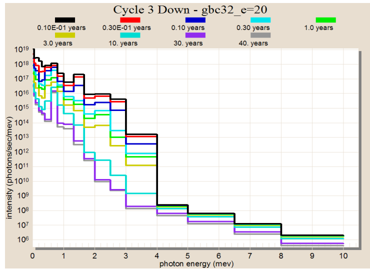
Figure 9: Gamma spectra in photons/s/MeV (e=2.0 w/o)
