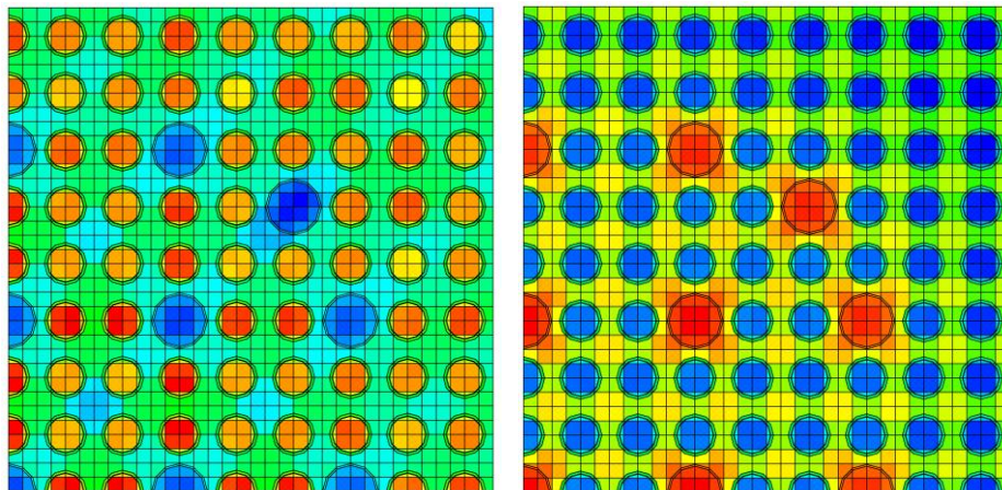
Figure 3: NEWT flux distribution over OFA model (left-first group, right-last group)
