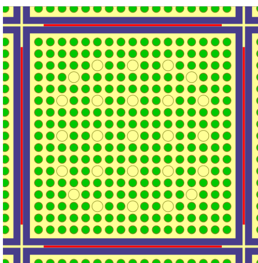
Figure 1: Cross sectional view of OFA cell inside GBC-32 cask
